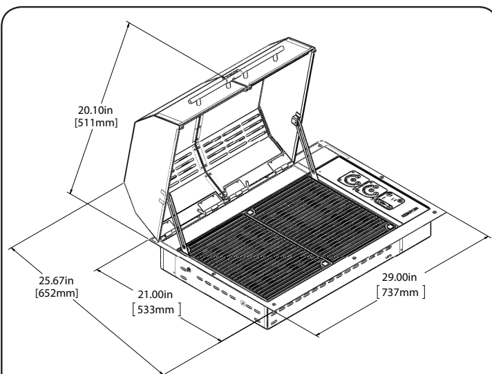
Overall Dimensions
